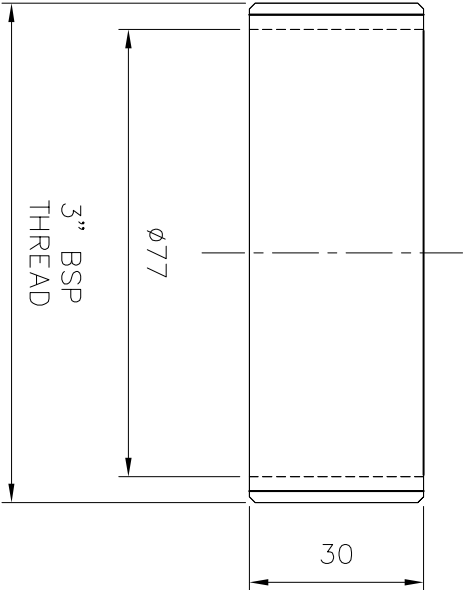
(SCALE-1:4) DETAIL-A BUSH FOR COUPLER
